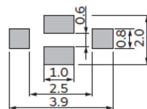
(in mm) NFM3DCC/3DPC
