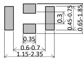
(in mm) NFM15PC105D0J3
