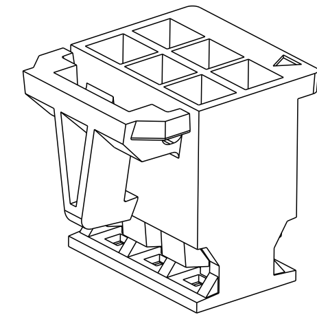
LATCH DESIGN FOR 10073599-006LF & 10073599-008LF ONLY
