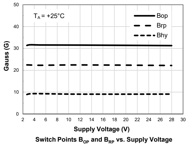
AH3322 Output Points (Magnetic Thresholds) – B_{OP} and B_{RP}
