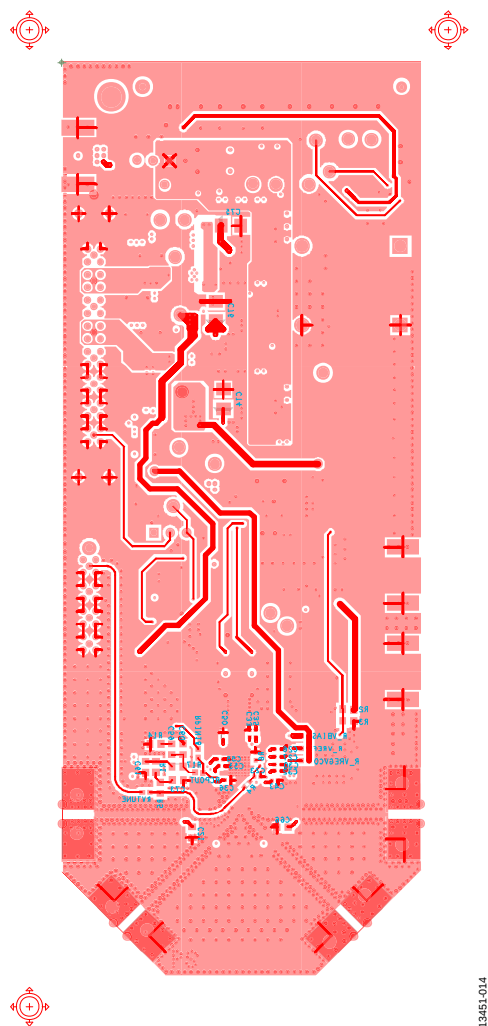
Figure 16. Evaluation Board Layer 4—Secondary
