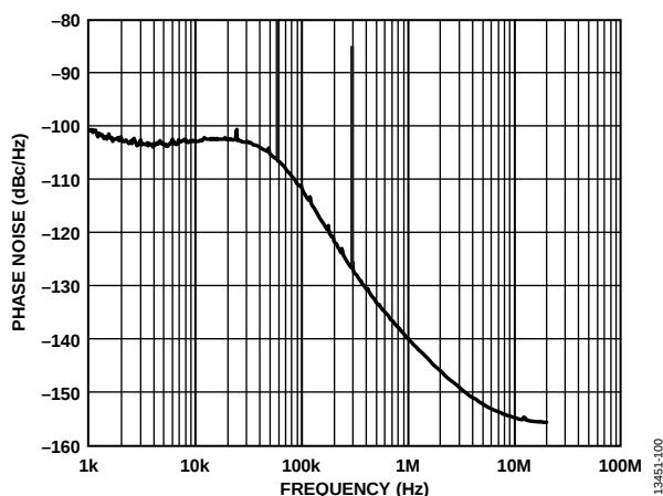
Figure 7. Single Sideband Phase Noise at 2113.5 MHz
