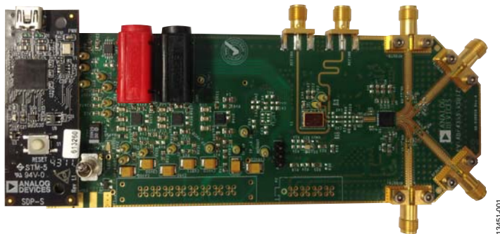
Figure 1. EV-ADF4355-3SD1Z
