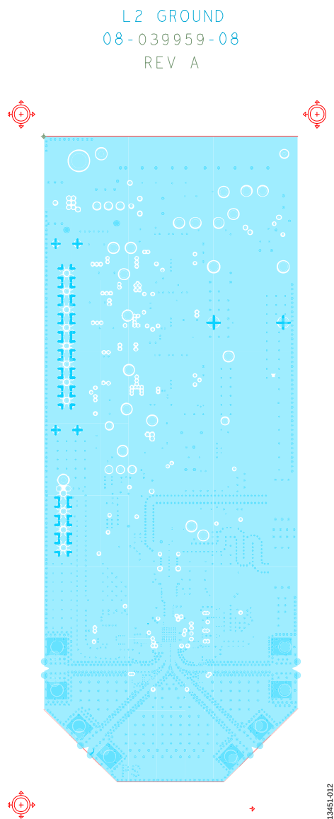
Figure 14. Evaluation Board Layer 2—Ground
