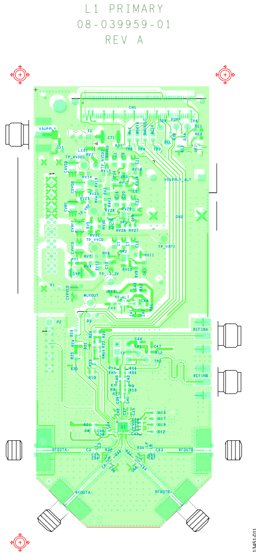
Figure 13. Evaluation Board Layer 1—Primary
