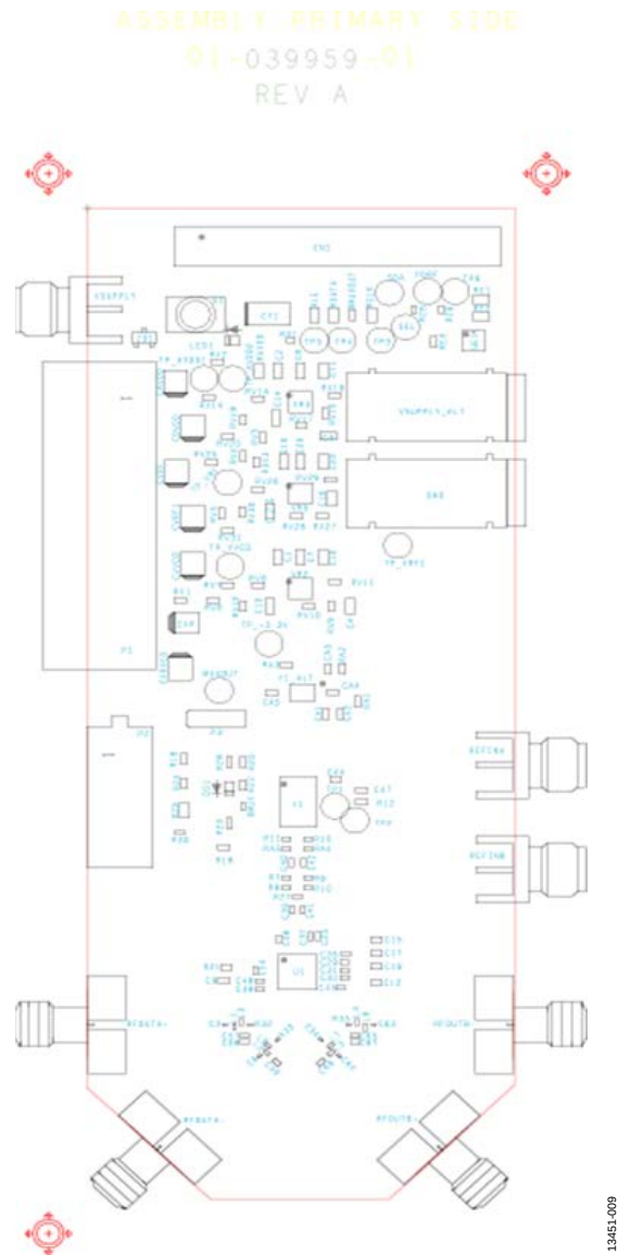
Figure 11. Evaluation Board Silk Screen—Top Side
