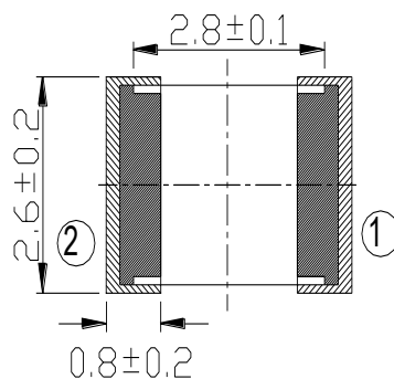
Recommended solder pad
