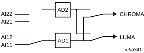
Fig 27. Mode 0; CVBS (automatic gain)
