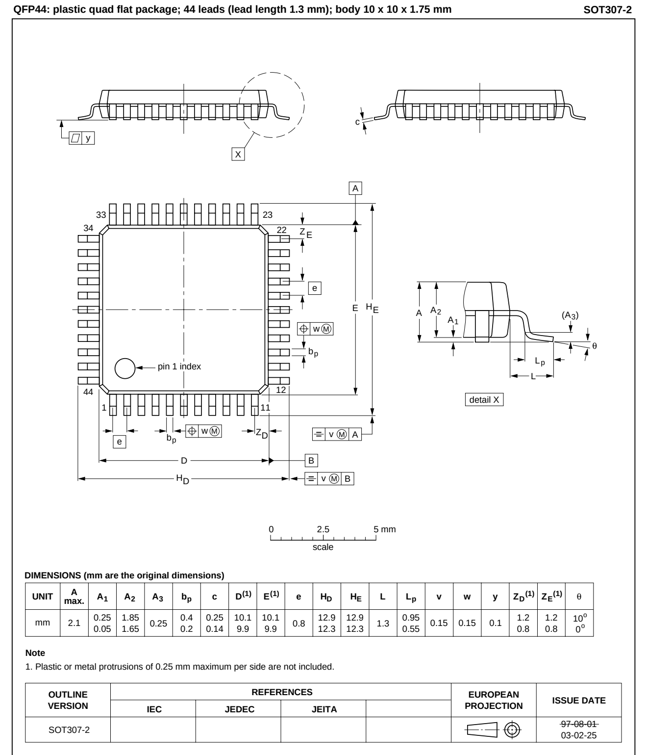
Fig 43. Package outline SOT307-2 (QFP44)
