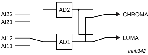
Fig 28. Mode 1; CVBS (automatic gain)
