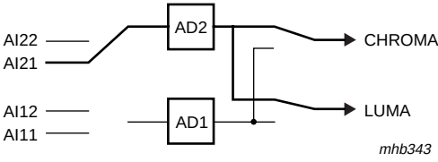
Fig 29. Mode 2; CVBS (automatic gain)
