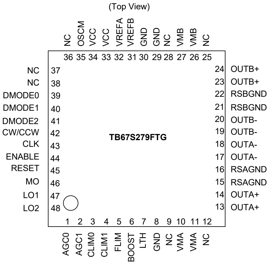
Figure 3.1 Pin Assignments
