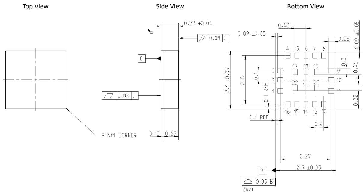
Figure 26: Outline dimensions
