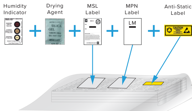
Vacuum bag.
