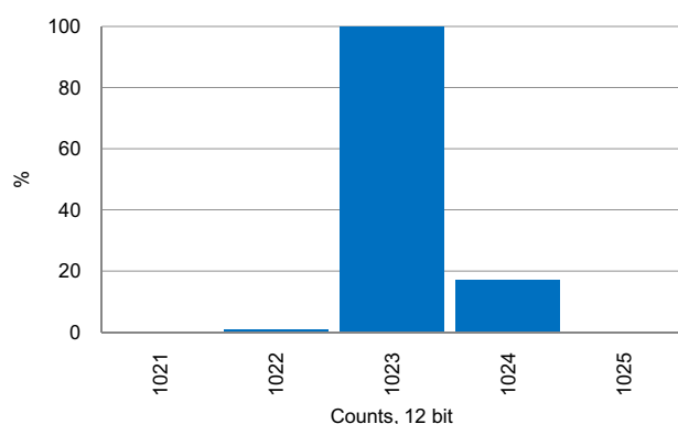
Figure 11-30. SAR ADC Noise Histogram, 1 mps, External
