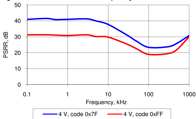
Figure 11-55. VDAC PSRR vs Frequency
