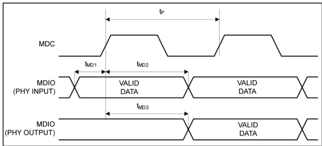
Figure 11. MDC/MDIO Timing
