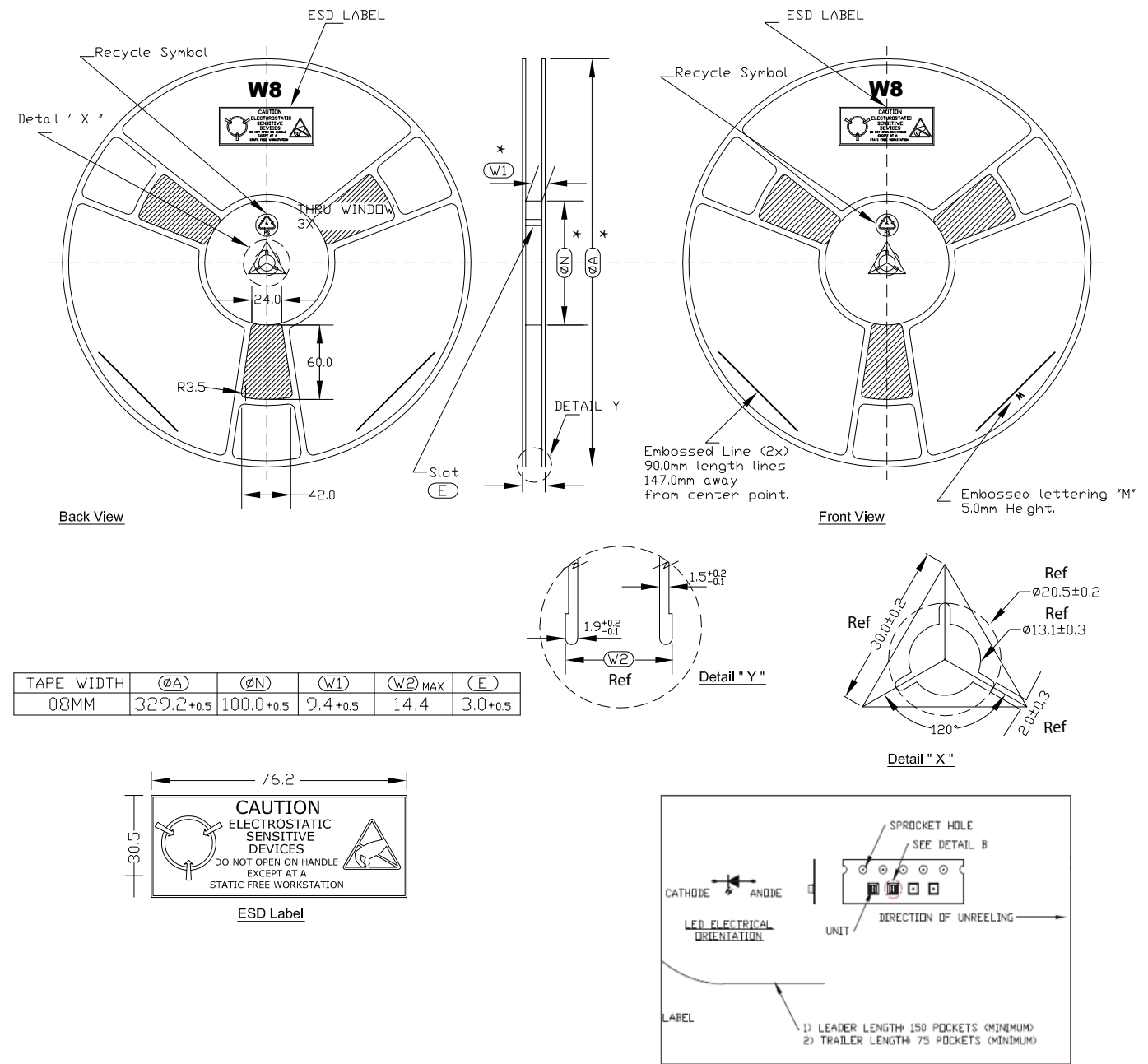
Figure 16. Reel dimensions for LUXEON CZ Color Line.
