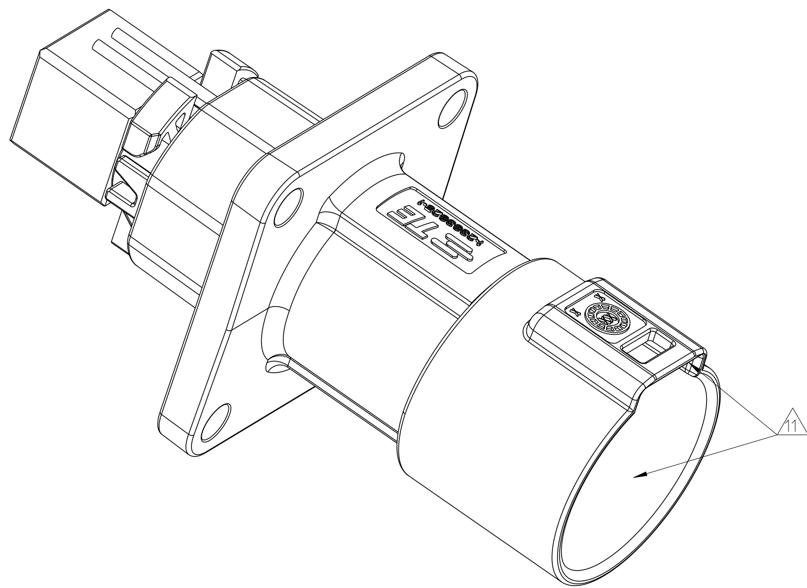
8-1 AS SHOWN
