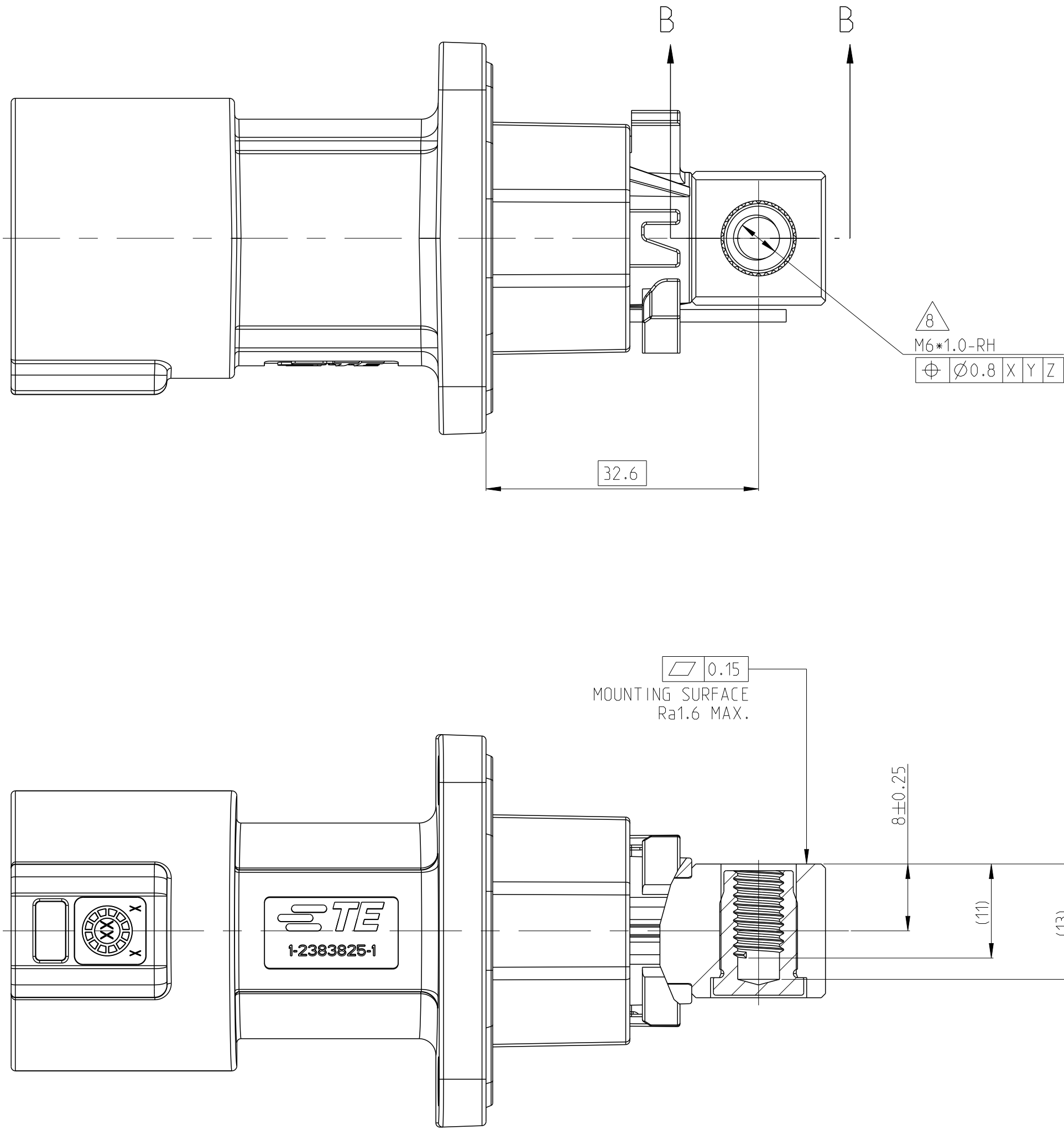
SECTION B-B
