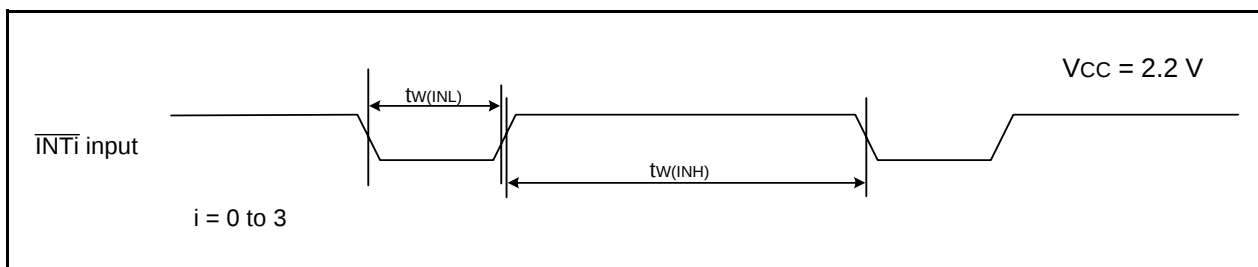
Figure 20.19 External Interrupt INTi Input Timing Diagram when Vcc = 2.2 V
