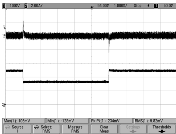
Step Load Transient Response@25°C (Vin=110V, Vout=nom., Iout=50-75-50% of fullload, Cload=0μF, ScopeBW =20MHz, 54mS/div)
