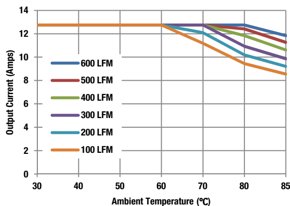
Maximum Current Temperature Derating (Vin = 110V)
