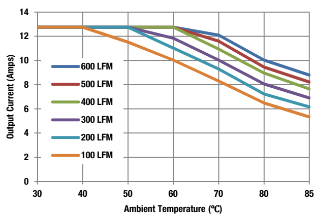
Maximum Current Derating (Vin = 160V)
