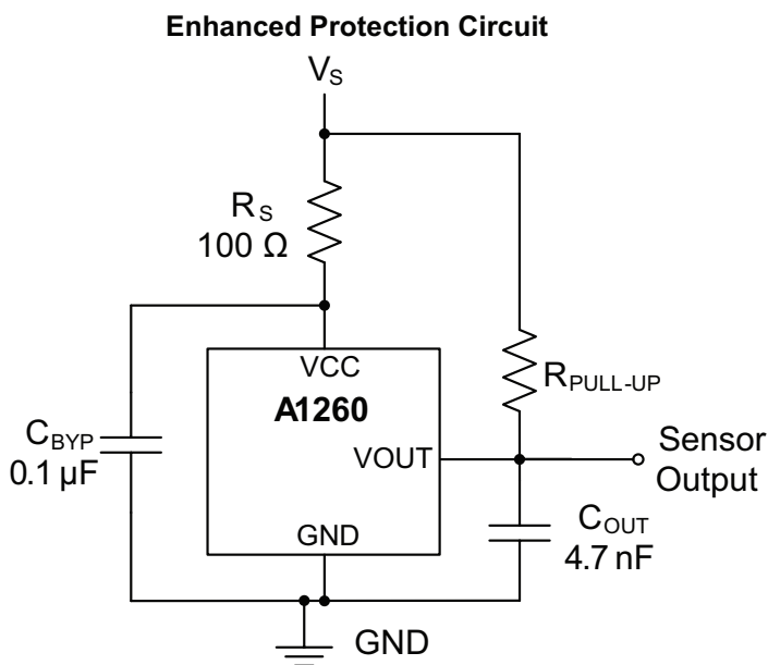
Figure 4: Typical and Enhanced Protection Application Circuits
