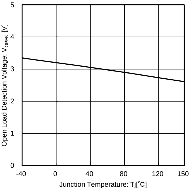
Figure 27. Open Load Detection Voltage vs Junction Temperature
