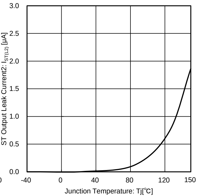
Figure 31. ST Output Leak Current2 vs Junction Temperature
