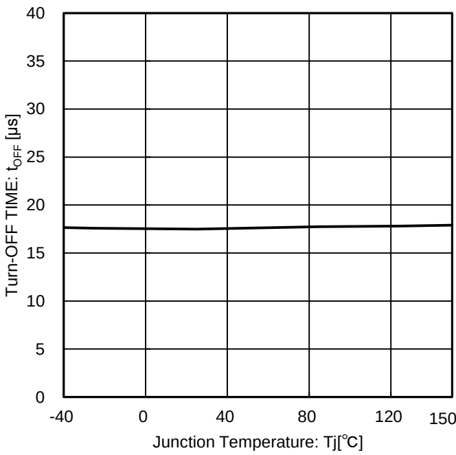
Figure 17. Turn-OFF TIME vs Junction Temperature
