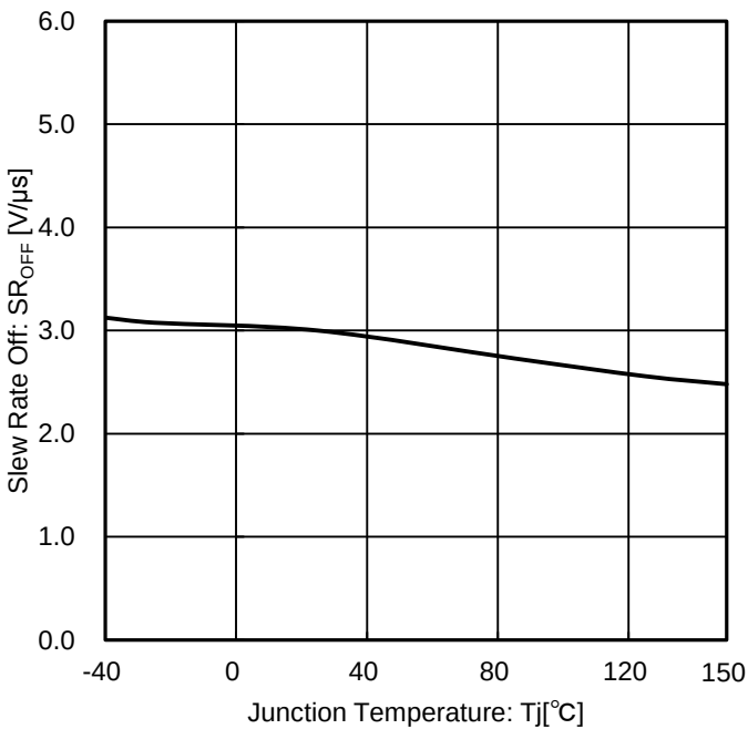
Figure 21. Slew Rate off vs Junction Temperature
