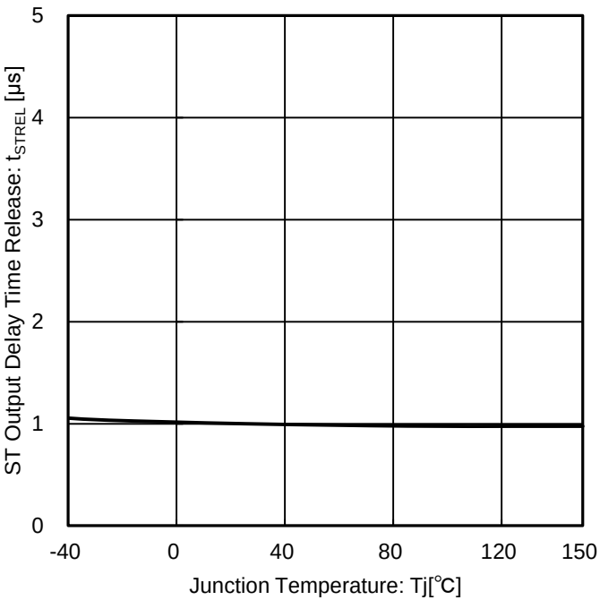
Figure 33. ST Output Delay Time Release vs Junction Temperature
