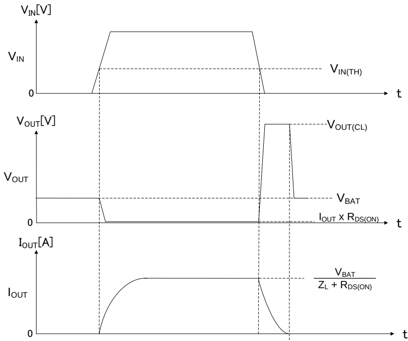
Figure 35. Inductive Load Operation
