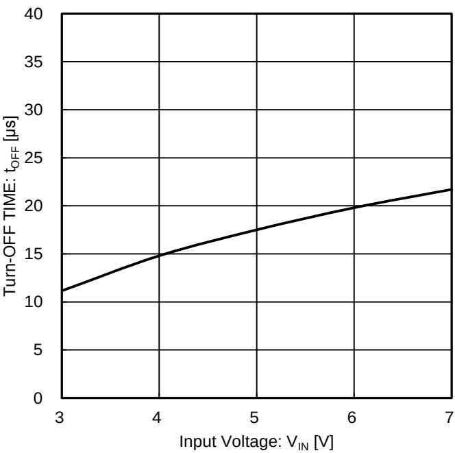
Figure 15. Turn-OFF TIME vs Input Voltage
