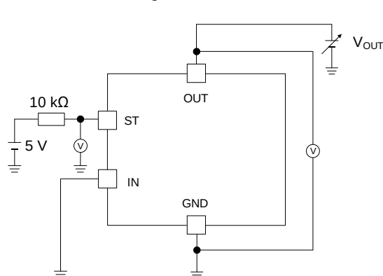
Measurement Circuit for Figure 27
