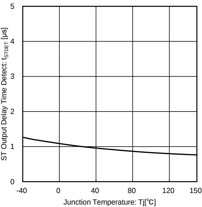
Figure 32. ST Output Delay Time Detect vs Junction Temperature
