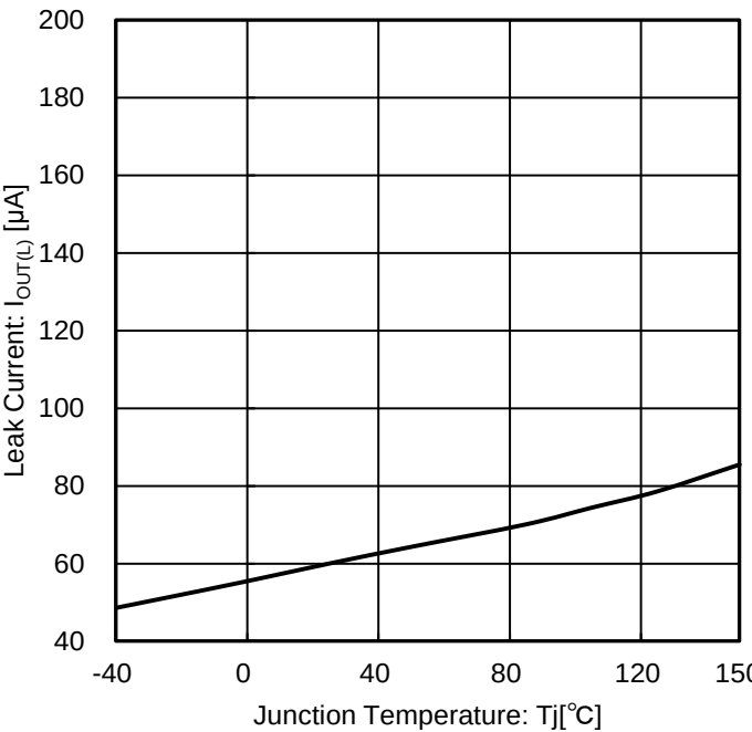
Figure 13. Leak Current vs Junction Temperature
