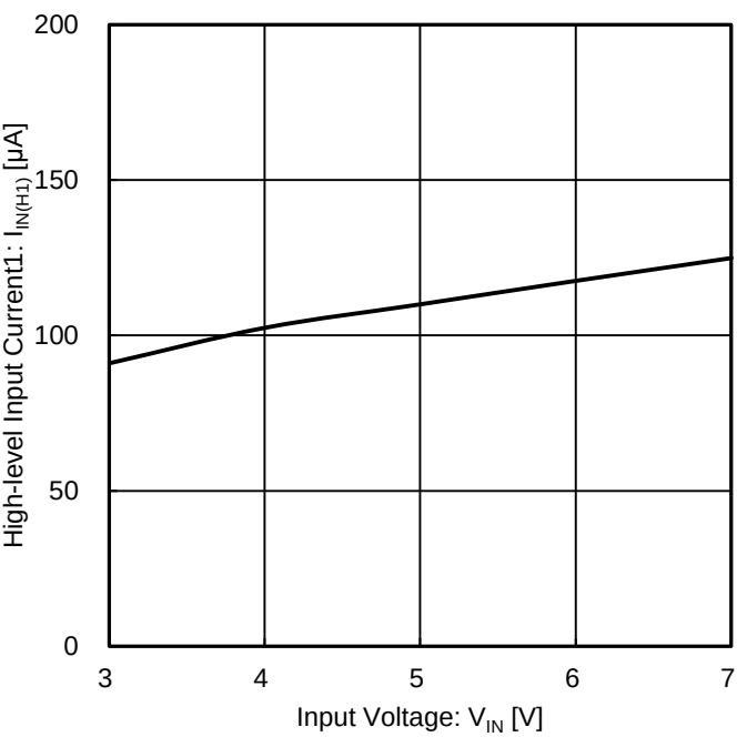
Figure 23. High-level Input Current1 (In Normal Operation) vs Input Voltage
