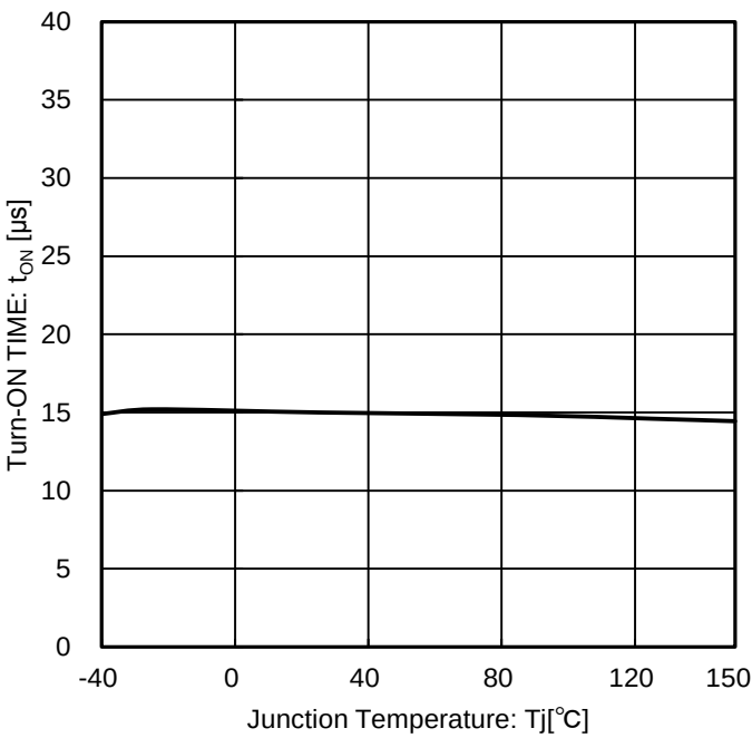
Figure 16. Turn-ON TIME vs Junction Temperature
