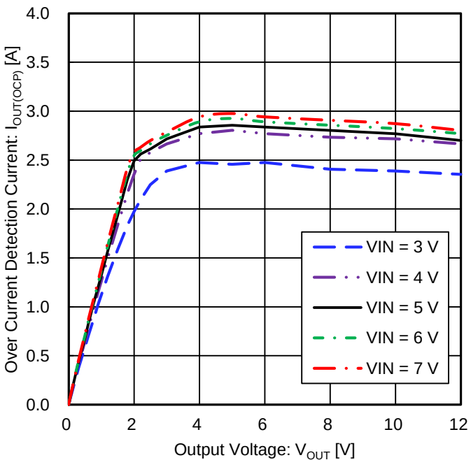
Figure 25. Over Current Detection Current vs Output Voltage
