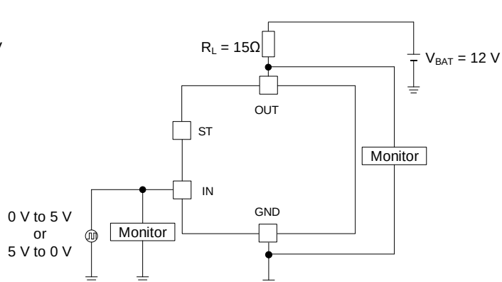
Measurement Circuit for Figure 14,15,16,17,18,19,20,21
