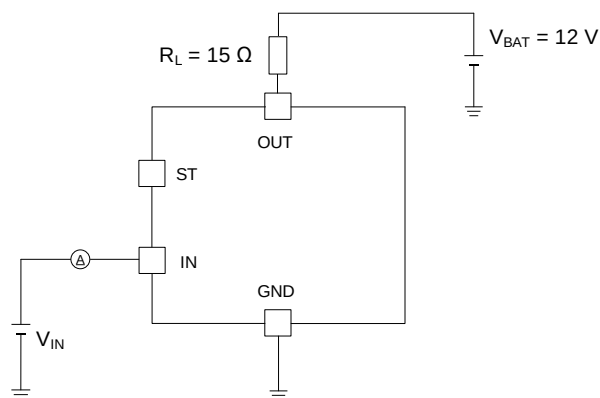
Measurement Circuit for Figure 23,24
