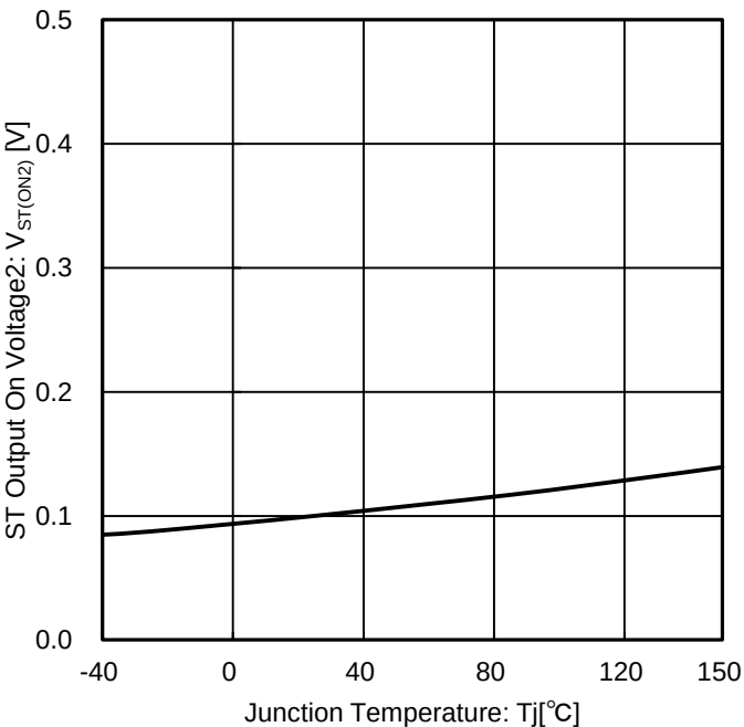
Figure 29. ST Output On Voltage2 vs Junction Temperature
