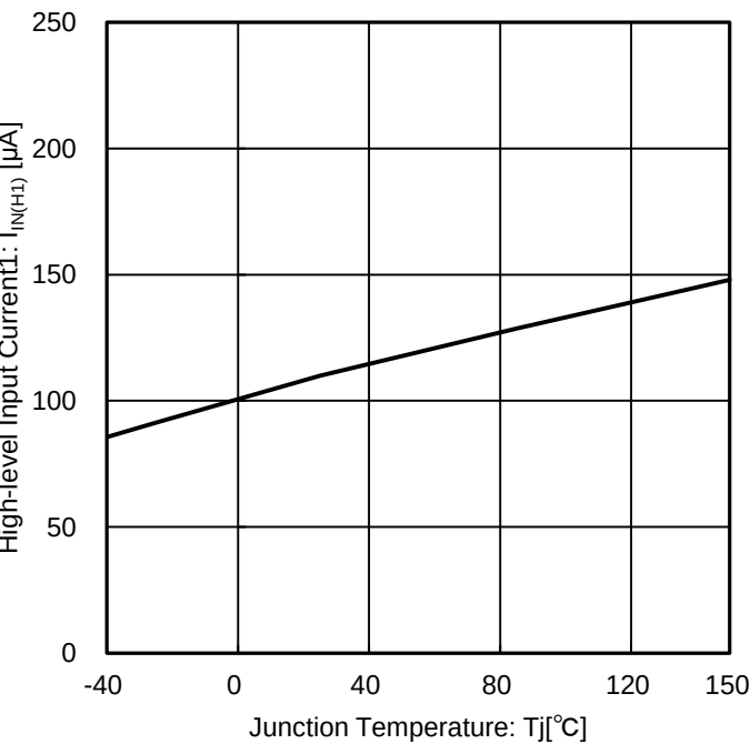
Figure 24. High-level Input Current1 (in Normal Operation) vs Junction Temperature
