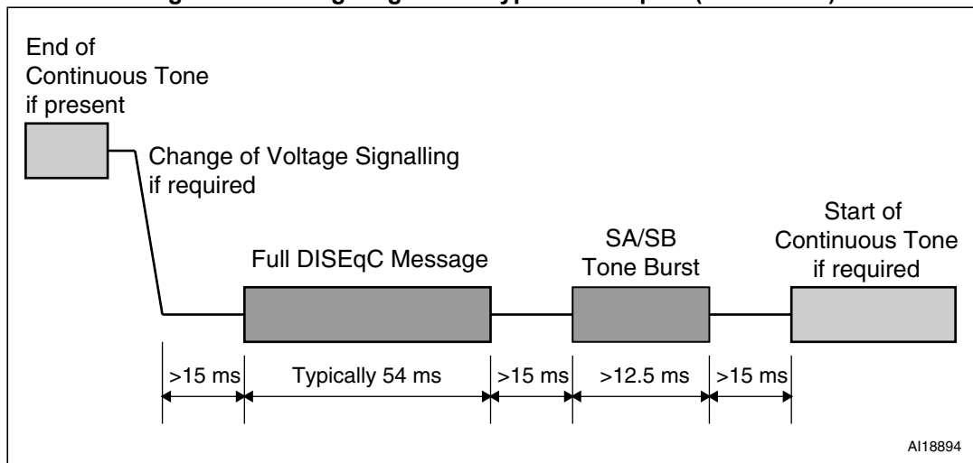
Figure 21. Timing diagram for typical DiSEqC™ (1.0 version)
