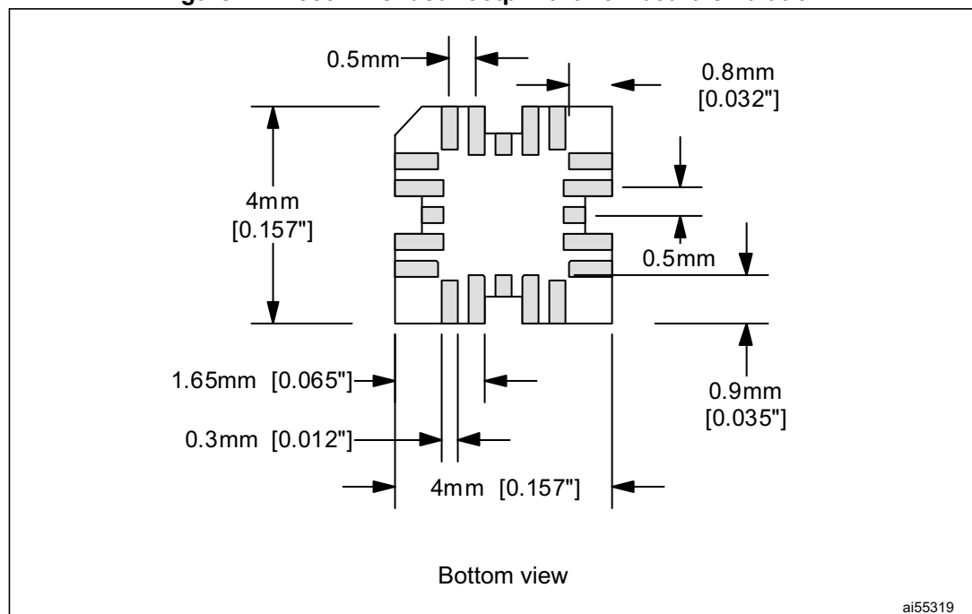
Figure 17. Recommended footprint for on-board emulation
