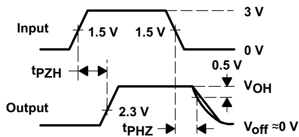
VOLTAGE WAVEFORMS
