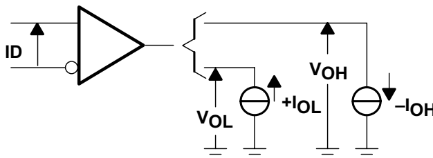
Figure 7-2. Receiver V_{OH} and V_{OL}
