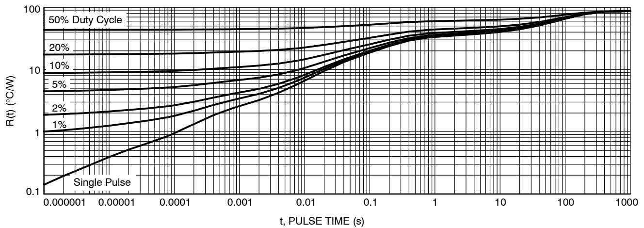
Figure 10. Thermal Characteristics
