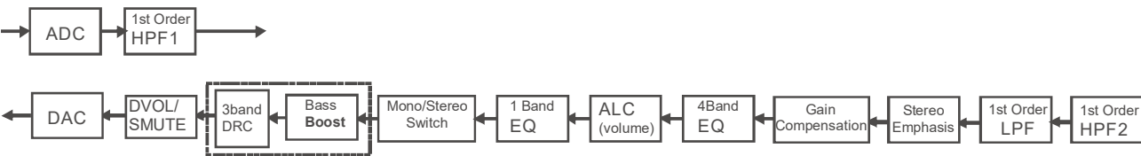
Figure 38. The Path in Recording Mode 2 & Playback Mode 1
