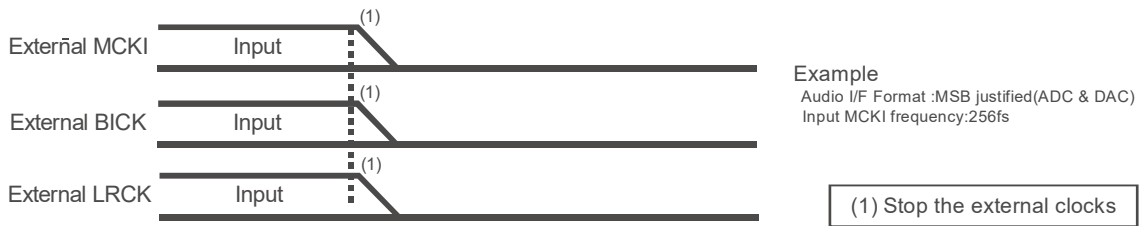
Figure 96. Clock Stopping Sequence (4)
