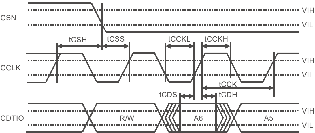
Figure 10. WRITE Command Input Timing
