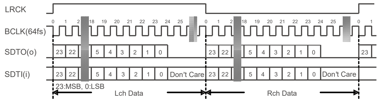
Figure 29. Mode 2 Timing
