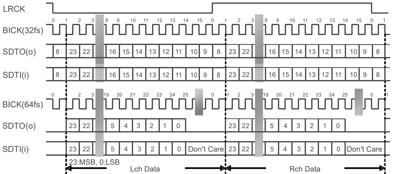
Figure 30. Mode 3 Timing
