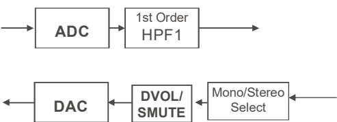
Figure 39. The Path in Recording Mode 2 & Playback Mode 2
