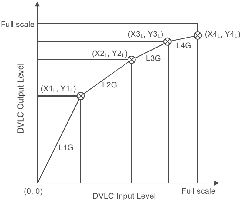
Figure 53. DVLC Curve for Low Frequency Range
