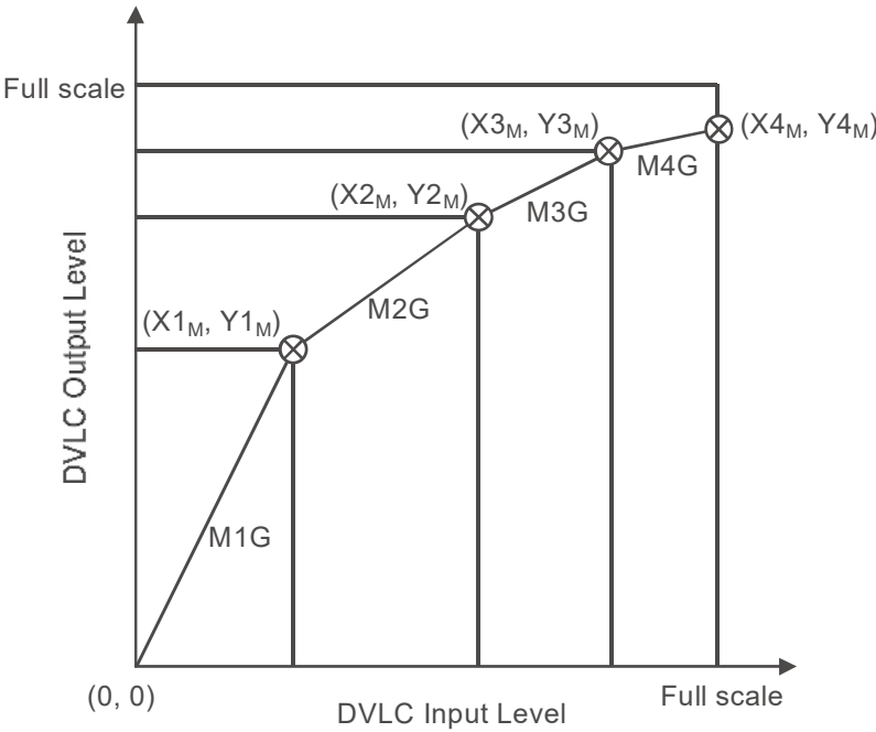
Figure 55. DVLC Curve for Middle Frequency Range
