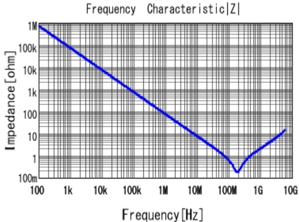
■ GRM155R71E222KA01 |Z| DC0V, 25degC
