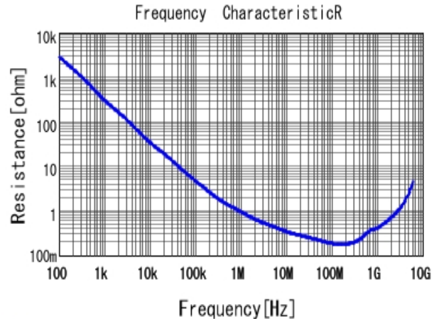
■ GRM155R71E222KA01 R DC0V, 25degC
