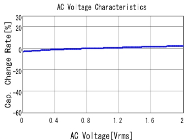
■ GRM155R71E222KA01 C-AC Voltage capchange, DC0V, 25.0d
