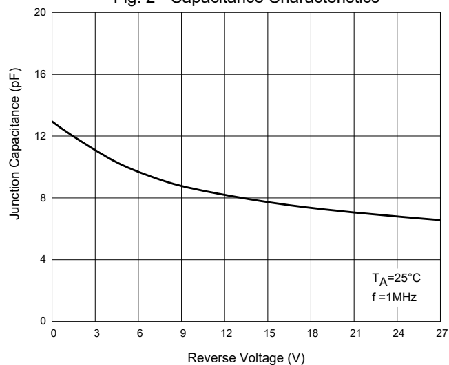
Fig. 2 - Capacitance Characteristics
