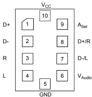
Figure 2. 10-Pin MicroPak™
