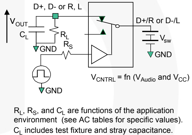
Figure 14. AC Test Circuit Load
