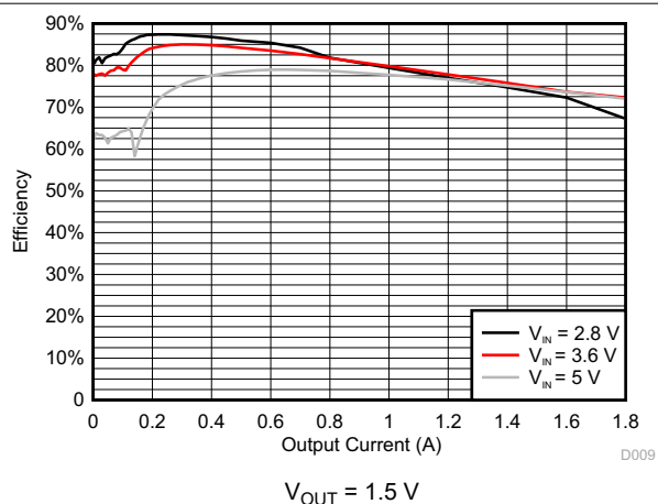
Figure 8-6. DCDC3 Efficiency
