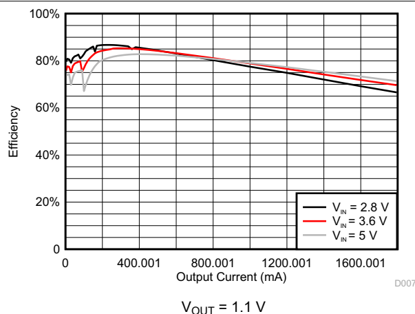
Figure 8-4. DCDC1/DCDC2 Efficiency
