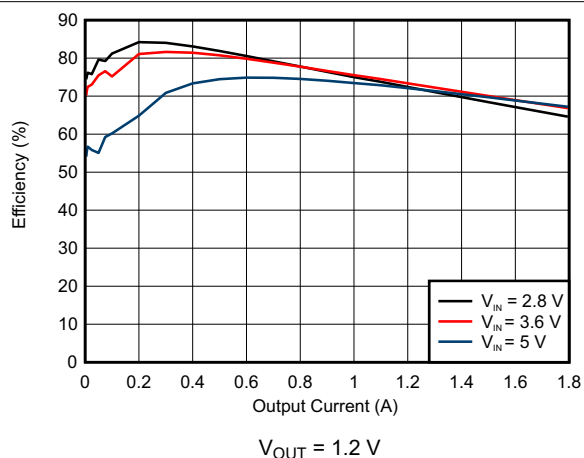
Figure 8-5. DCDC3 Efficiency
