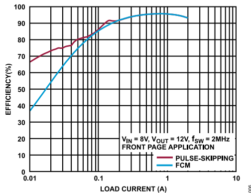
Figure 3. Efficiency vs Load Current (Boost Region)
