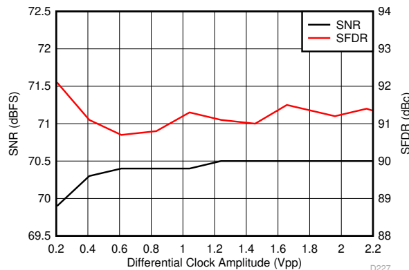
Figure 6-117. Performance vs Differential Clock Amplitude (40 MHz)
