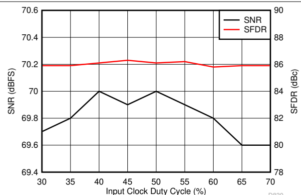
Figure 6-30. Performance vs Clock Duty Cycle (150 MHz)
