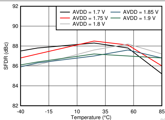
Figure 6-113. Spurious-Free Dynamic Range vs AVDD Supply and Temperature (170 MHz)
