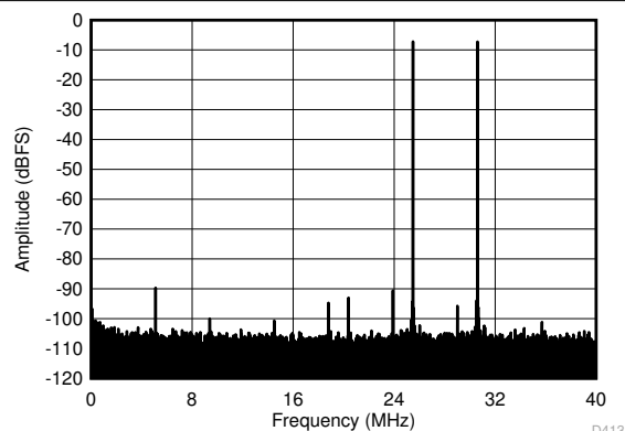
Figure 6-73. FFT FOR Two-Tone Input Signal ( -7\text{ dBFS} at 185 MHz and 190 MHz)
