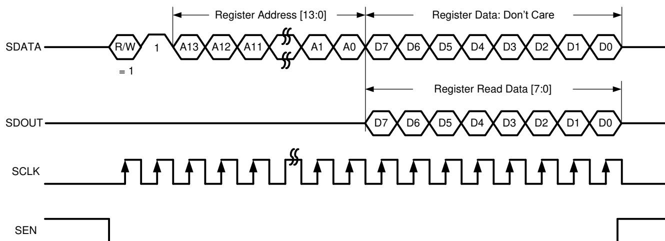
Figure 8-14. Serial Register Read Timing Diagram
