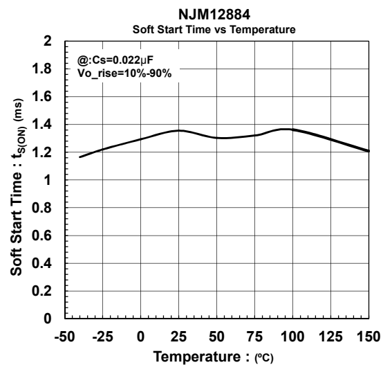
Soft-Start Time (0.022 \mu\text{F} ) vs. Temperature
