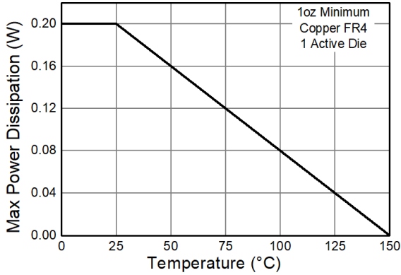
Fig 1. Derating Curve
