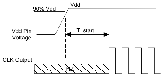
Figure 11. Startup Timing
