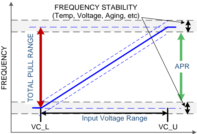
Figure 26. Typical SiTime VCTCXO FV Characteristic
