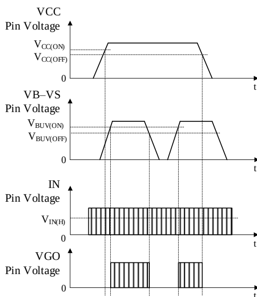
Figure 8-2. Operational Waveforms
