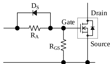
Figure 8-5. Power MOSFET Peripheral Circuit
