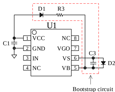
Figure 8-4. Bootstrap Circuit
