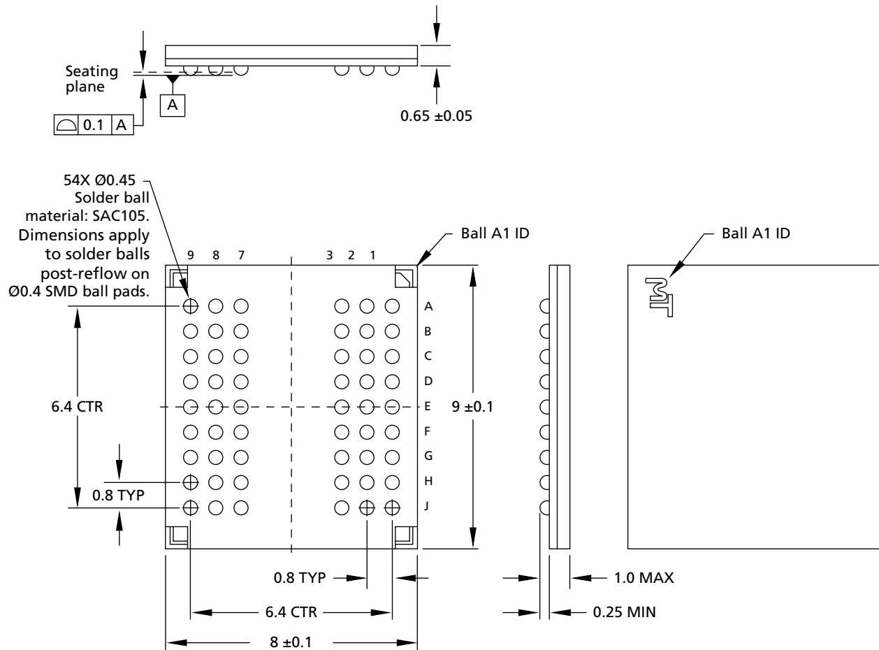
Figure 5: 54-Ball VFBGA (8mm x 9mm)
