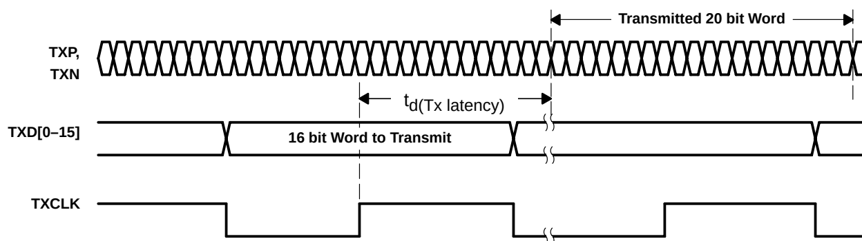
Figure 3. Transmitter Latency
