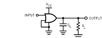
FIGURE 1. AC Test Circuit
