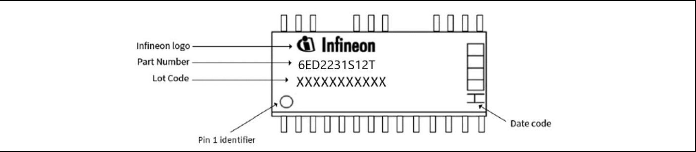
Figure 31 Marking information PG-DSO-24 (DSO-28 with 4 pins removed) [Marking Diagram to be updated]
