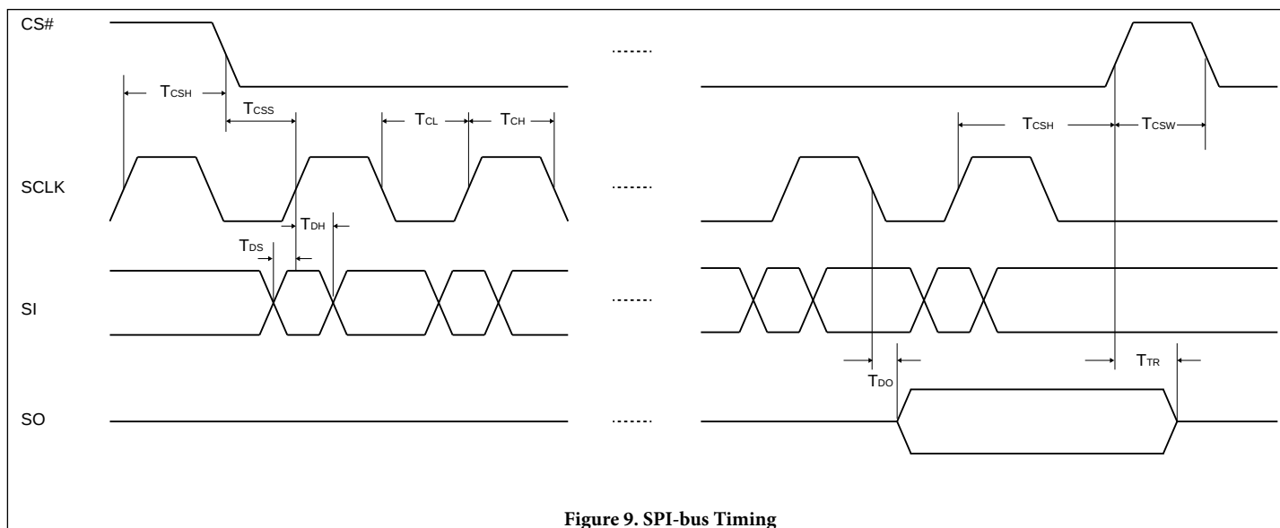
Figure 9. SPI-bus Timing
