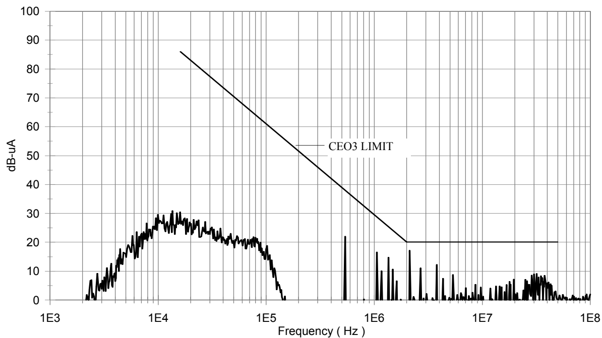
Fig 3. Conducted Emissions, Positive Lead
