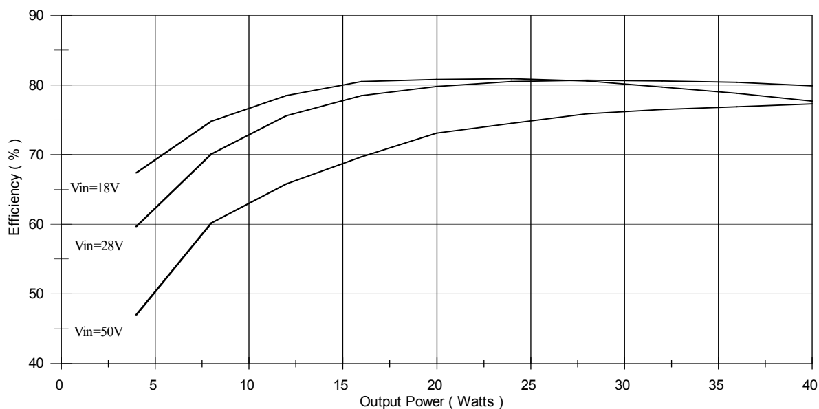
Fig 7. M3G2812S Efficiency
