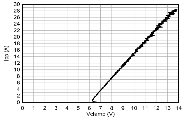
Figure 6-2. Negative TLP Curve
