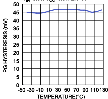
PG Hysteresis vs. Temperature
