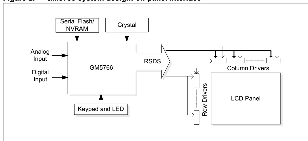
Figure 2. GM5766 system design: on-panel interface
