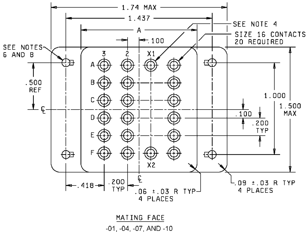
FIGURE 1. Socket configurations.
