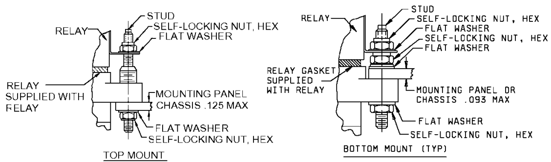
FIGURE 2. Recommended mounting dimensions.
