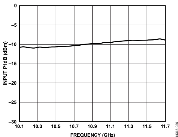
Figure 17. Input P1dB vs. Frequency
