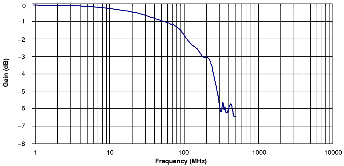
Figure 8. Frequency Response ( C_L = 0\text{ pF} , V_{CC} = 3.3\text{ V} )
