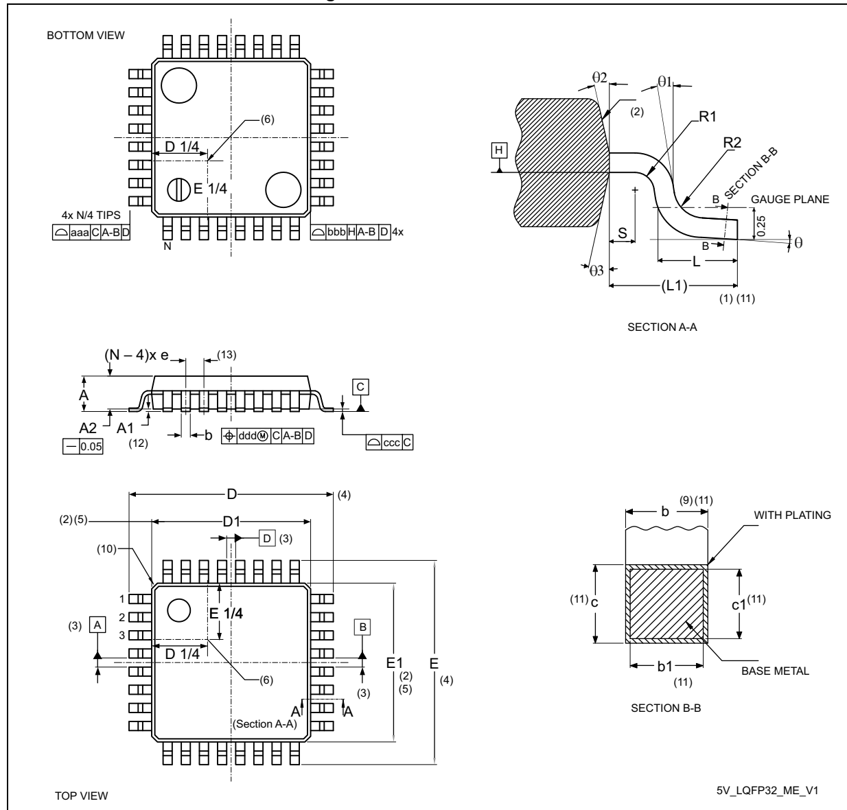
Figure 41. LQFP32 - Outline
