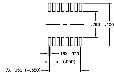
SUGGESTED LAND PATTERN
