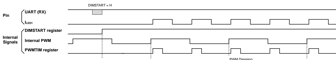
Figure 49. PWMFREQ = 1
