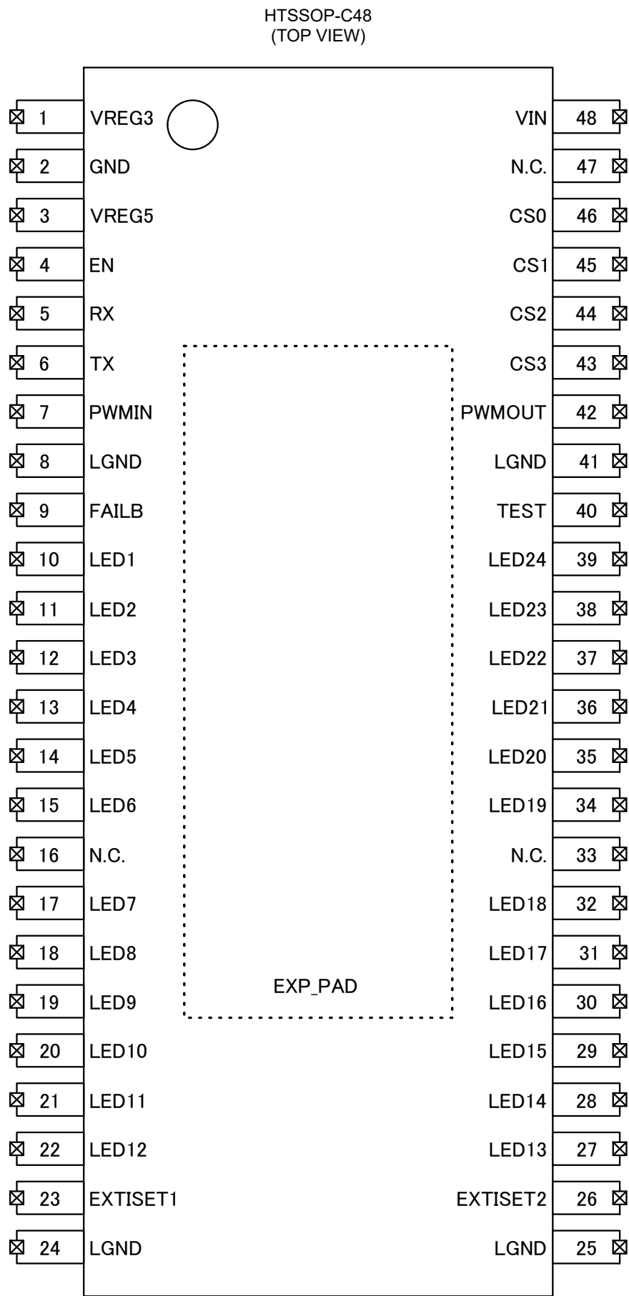
Figure 2. Pin Configuration
