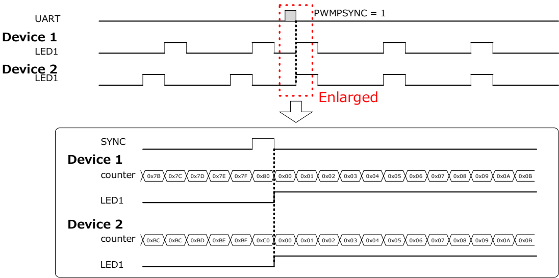
Figure 37. SYNC Register Setting Function
