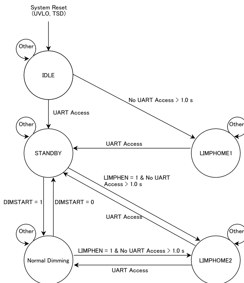
Figure 9. LIMPHOME Function
