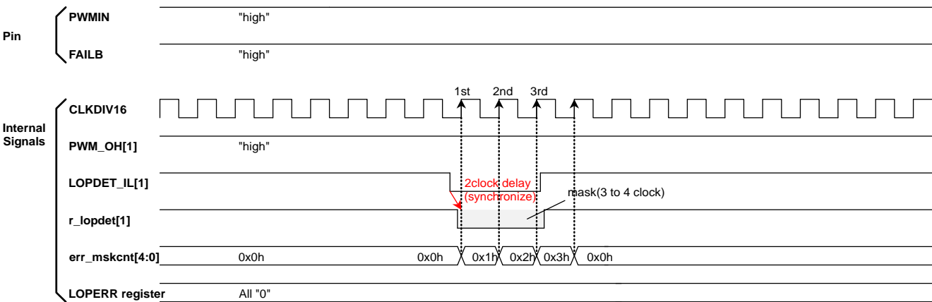
Figure 64. LED Open Protection Masked (Enlarged View A)
