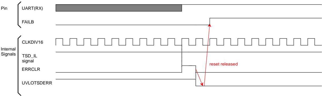
Figure 54. TSD Released Function (Enlarged View B)
