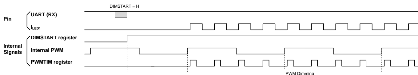
Figure 50. PWMFREQ = 2
