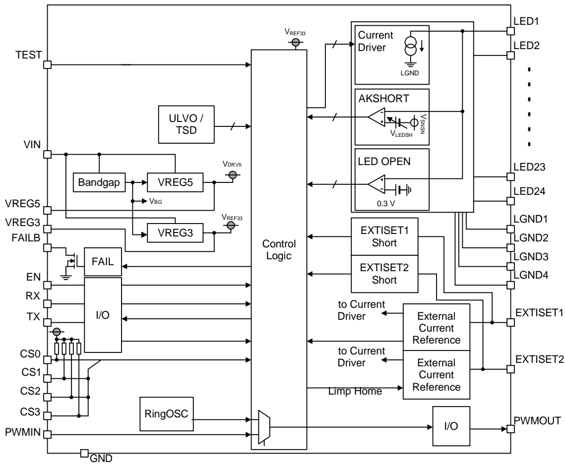
Figure 3. Block Diagram
