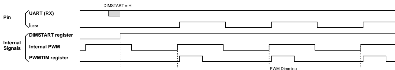
Figure 48. PWMFREQ = 0
