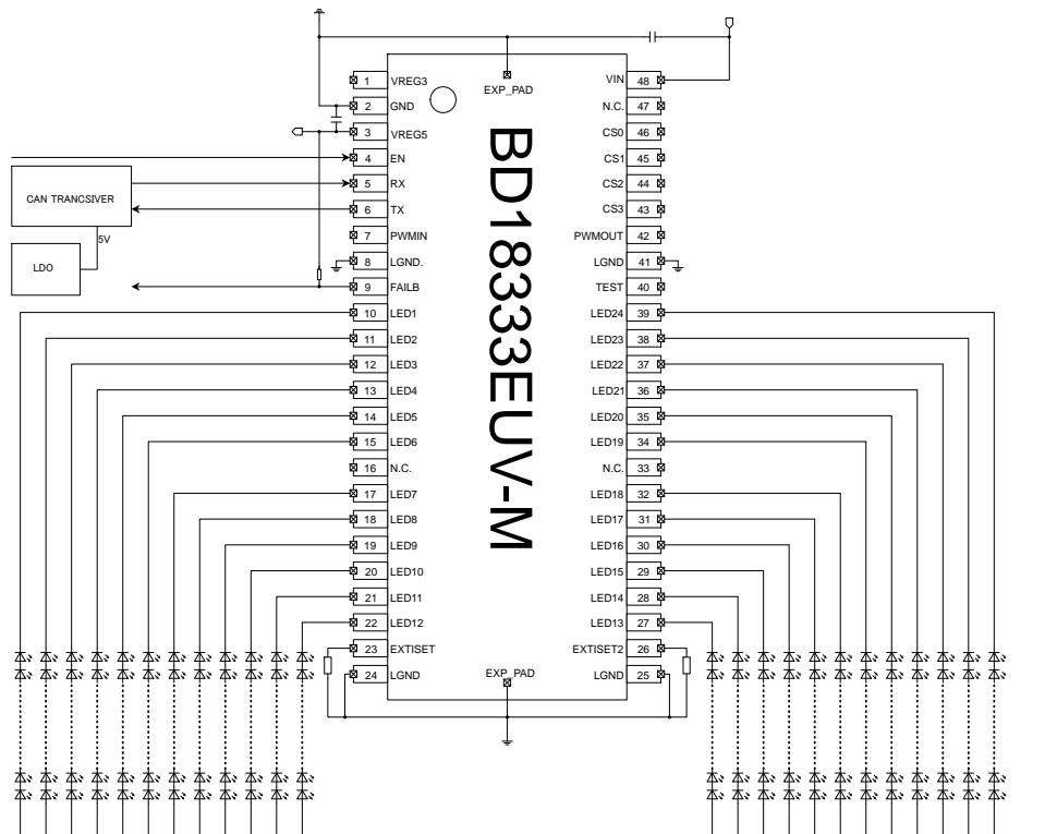
Figure 1. Application Circuit
