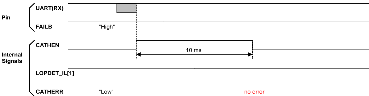
Figure 67. LED Cathode Short Protection (No Error)
