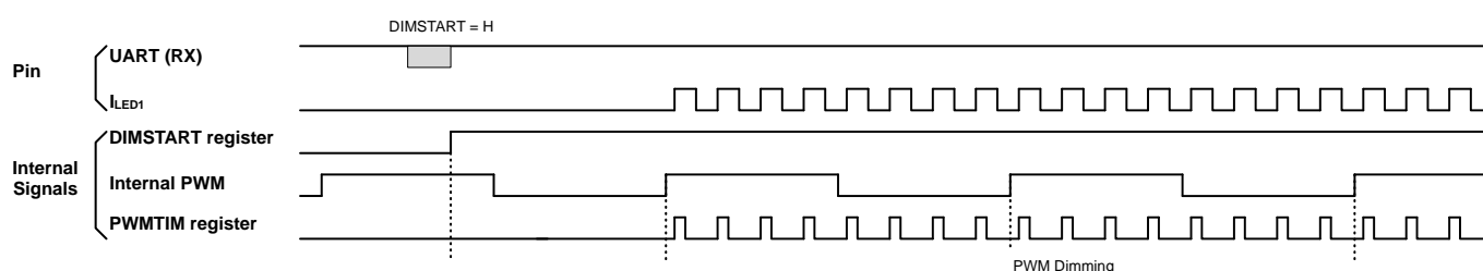
Figure 51. PWMFREQ = 3
