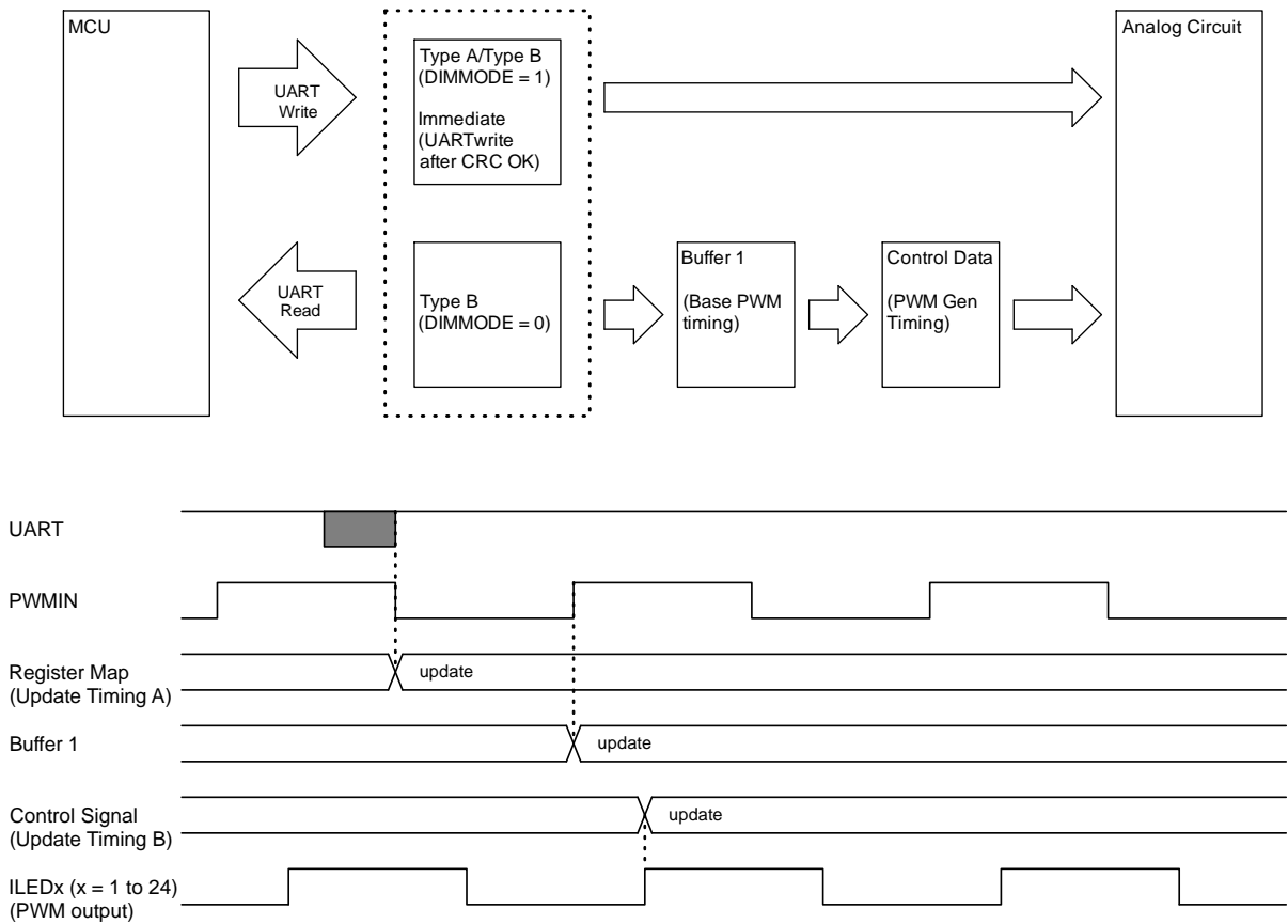
Figure 30. UART Data Flow
