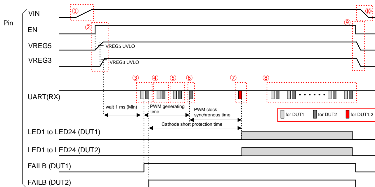
Figure 75. Starting Sequence for Normal Operation
