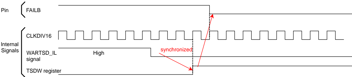
Figure 56. TSD Warning Detected Function (Enlarged View A)
