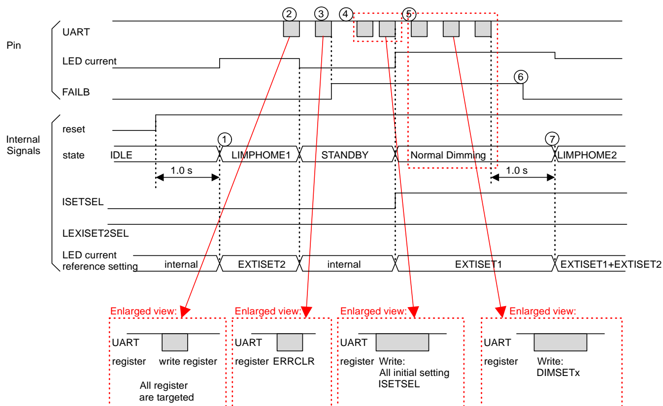
Figure 88. LIMPHOME Function Sequence (Case2)
