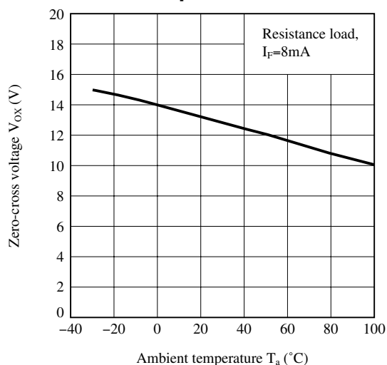
Fig.10 Zero-cross Voltage vs. Ambient Temperature
