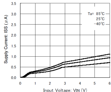
Supply Current vs. Input Voltage IXD5120x272xx
