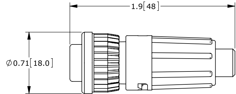
SHOWN ASSEMBLED WITH STANDARD COUPLING RING
