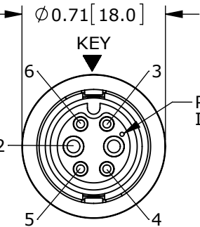
MATING FACE ASSY: W6C80-6PG-522 SHOWN
