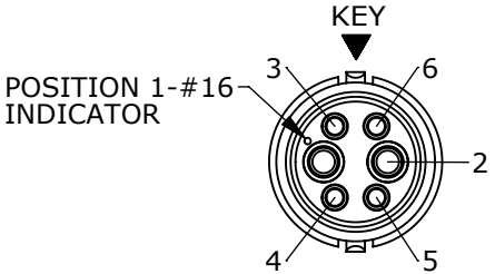
WIRING END ASSY: W6C80-6PG-522 SHOWN
