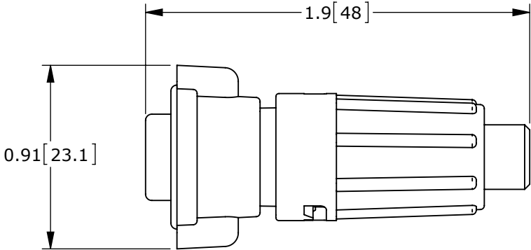
SHOWN ASSEMBLED WITH WIMGED COUPLING RING
