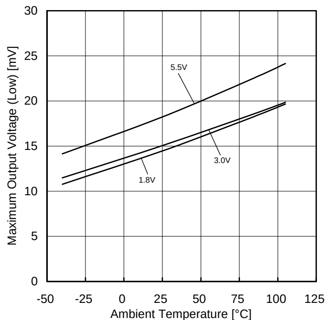
Figure 28. Maximum Output Voltage (Low) vs Ambient Temperature ( R_L=10k\Omega )
