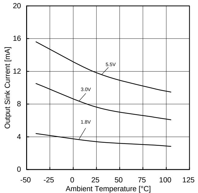
Figure 10. Output Sink Current vs Ambient Temperature (OUT=VSS-0.4V)
