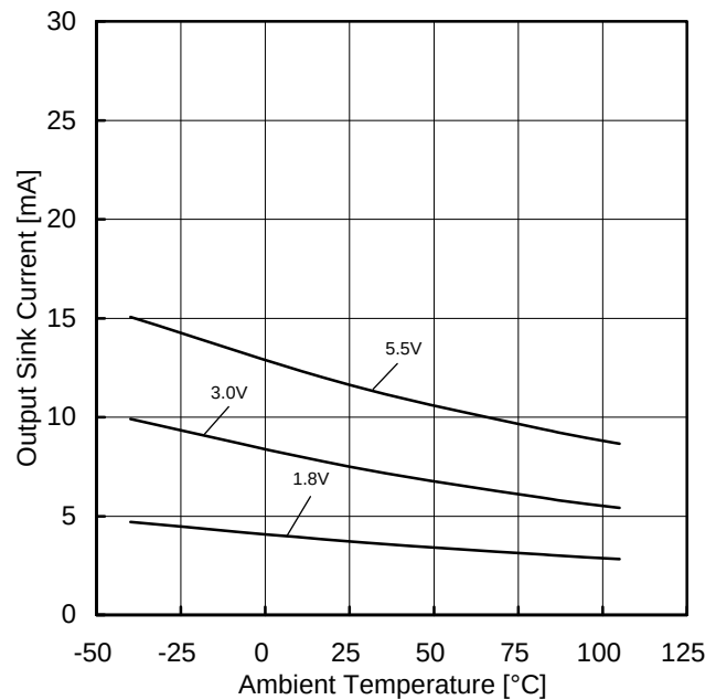
Figure 30. Output Sink Current vs Ambient Temperature (OUT=VDD-0.4V)
